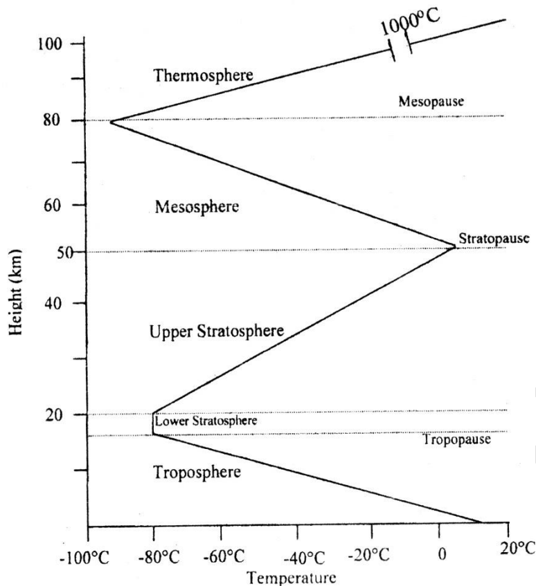
TEMPERATURE BASED VERTICAL LAYERS OF ATMOSPHERE
