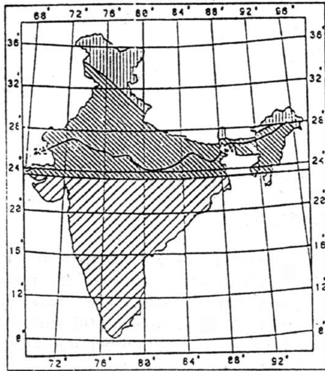
Climate zones based on Temperature
